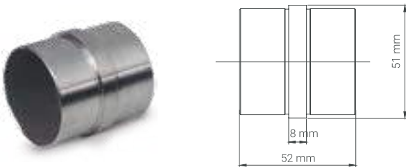
Empalme tubo interior
