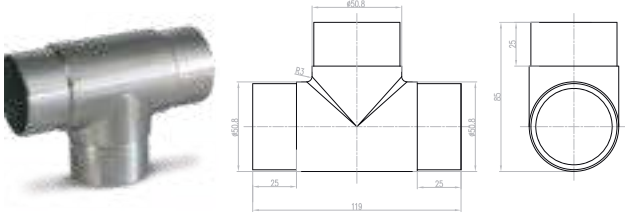
Empalme tee tubo interior
