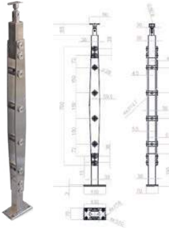
Balaustre planchuela p/tubo o barra \varnothing 12 mm
